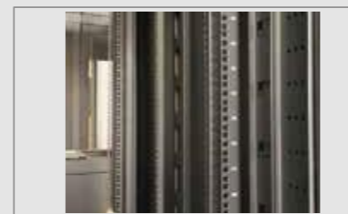
Front (rear) sides of cabinet with vertical PDU and wire trimmers
