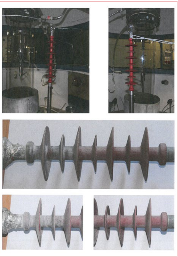
VEIKI 5000 h ageing test for composite insulators
